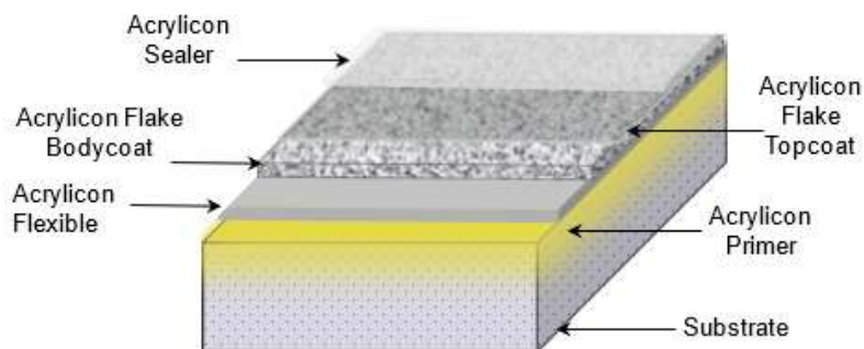
Figur 2: AcryliCon Flake System
